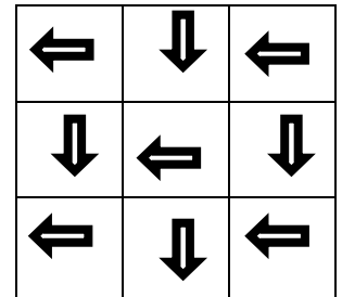
Checkerboard Style
